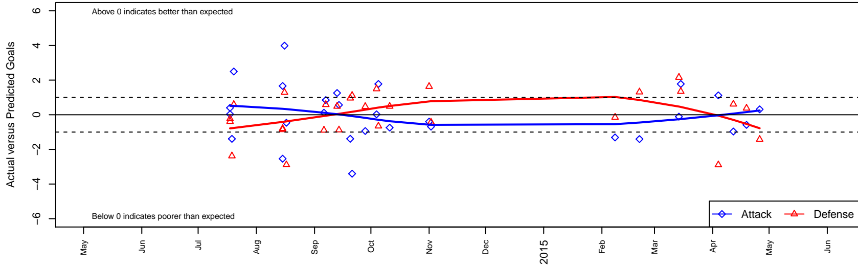
HSC Blaze G02 Dots are actual minus expected GF (blue circles) and GA (red triangles). Blue line is smoothed change in attack strength. Red is smoothed change in defense strength.
